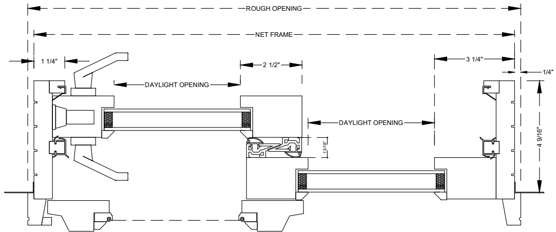
Jambs and Interlock
