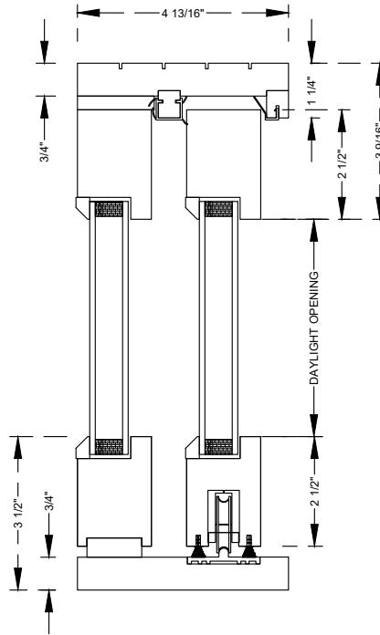
Head & Sill
