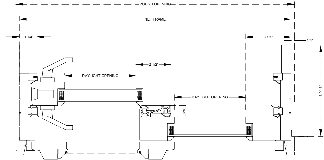
Jambs and Interlock
