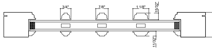
1/2" Long Bead Interior/Long Bead Exterior
