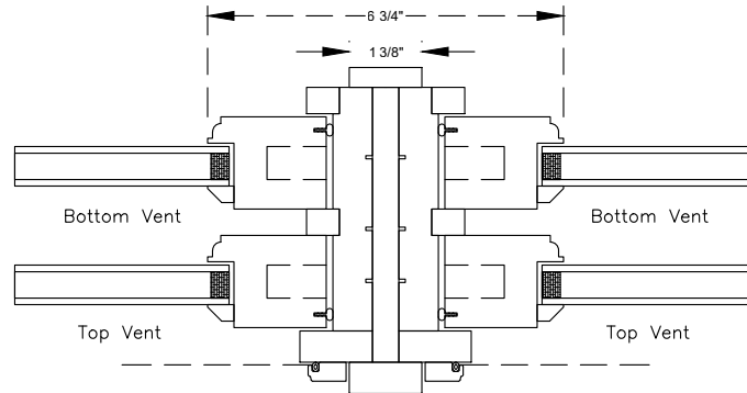
Standard Stack Mull
