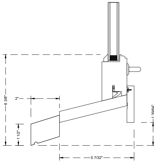
True Subsill Match (2816)
