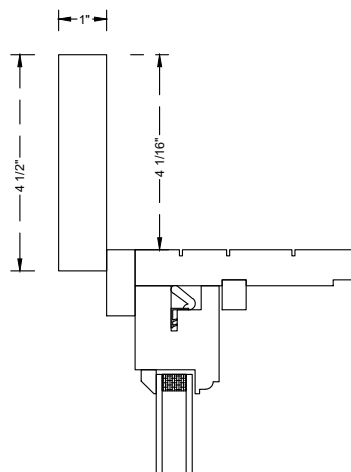
5/4 x 5 Casing
