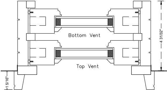
1 5/16 Setback Nail Fin* *Not compatible with brickmold or subsills
