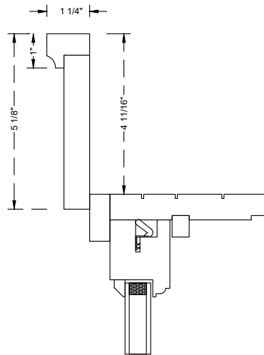
1 x 5 Casing w/ Backband
