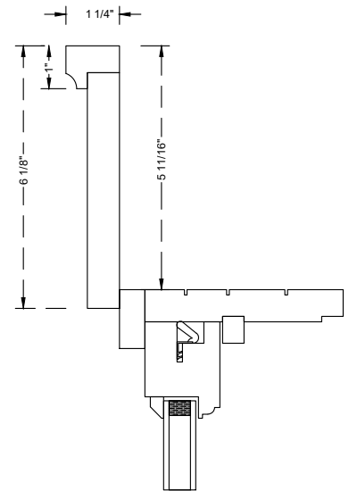
1 x 6 Casing w/ Backband
