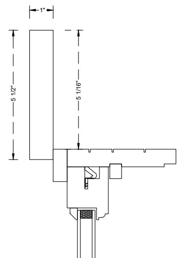
5/4 x 6 Casing
