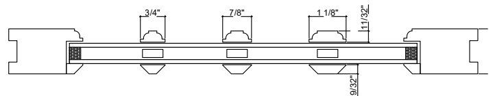
3/8" Long Bead Interior/Bevel Bead Exterior *
