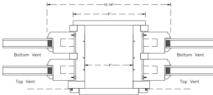
4" Space Mull
