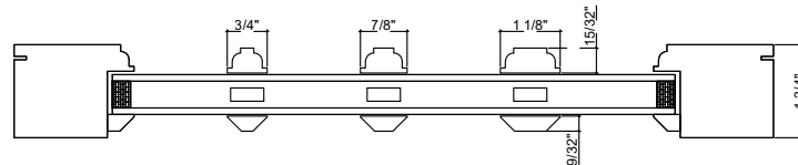
1/2" Long Bead Interior/Bevel Bead Exterior
