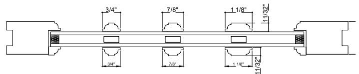
3/8" Long Bead Interior/Long Bead Exterior *
