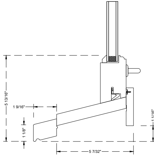
Standard Subsill (2814)
