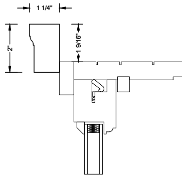
Brickmold Casing
