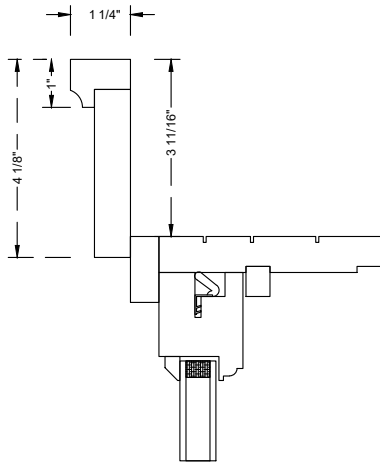
1 x 4 Casing w/ Backband
