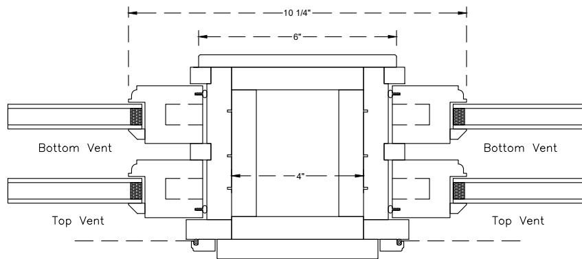
4" Spread Mull
